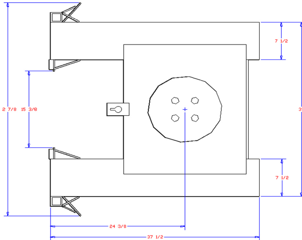
LIFTOMATIC L4F Based on 500kg per drum (1102 lbs)
